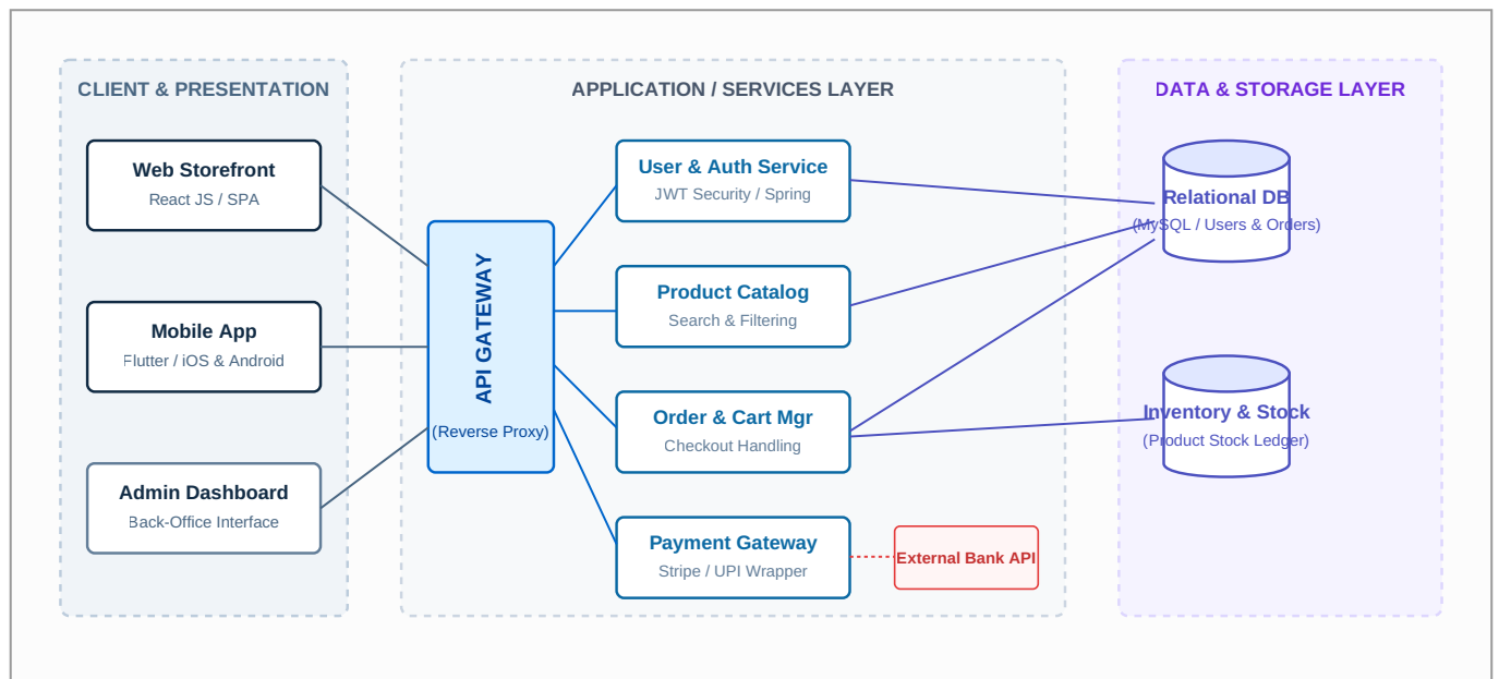
Figure 1: Architecture and data flow of the ShopEZ e-commerce sample application
